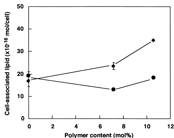
Fig. 3. Influence of the amount of the grafted polymer on uptake by CV1 cells at 37 (●) and 42°C (◆) in DMEM. The bars represent the S.D. ( n=3 ). The concentration of liposomal lipid in the incubation was 0.6 mM.
