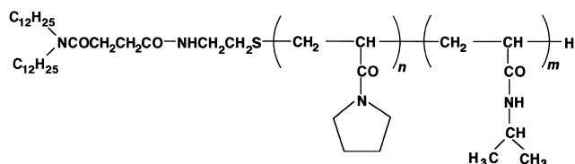
Fig. 1. Structure of poly(APr-co-NIPAM)-2C 12 .
